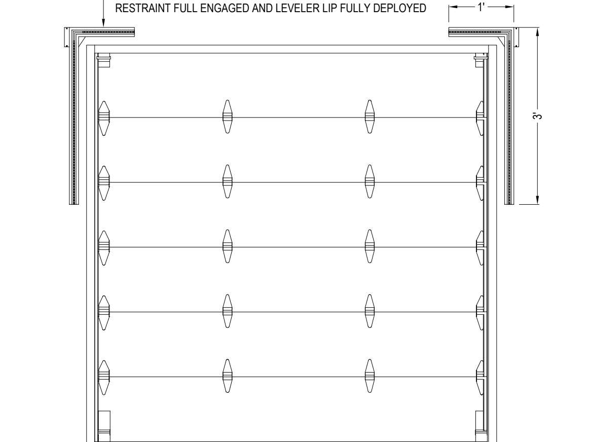
ELEVATION LOADING DOCK SAFETY LIGHT INSTALLATION
